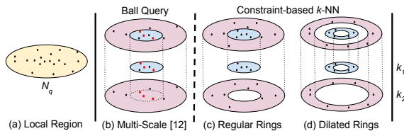
Figure 1: A schematic comparison for searching neighbors in a local region with N_q points between multi-scale approach from [12] and our proposed approaches with regular and dilated rings. The number of neighboring points per region (e.g., k_1 and k_2 ) is the same between different methods. Regions in multi-scale architecture have neighboring overlaps (red points belong to different regions near the same query point q ), while regular and dilated rings have the unique neighbors.
