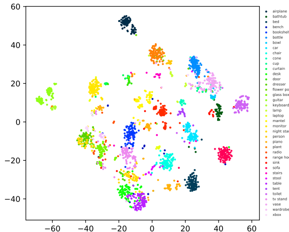
Figure 5: The t-SNE clustering visualization of the learned global shape features from the proposed A-CNN model for the shapes in ModelNet40 test split.
